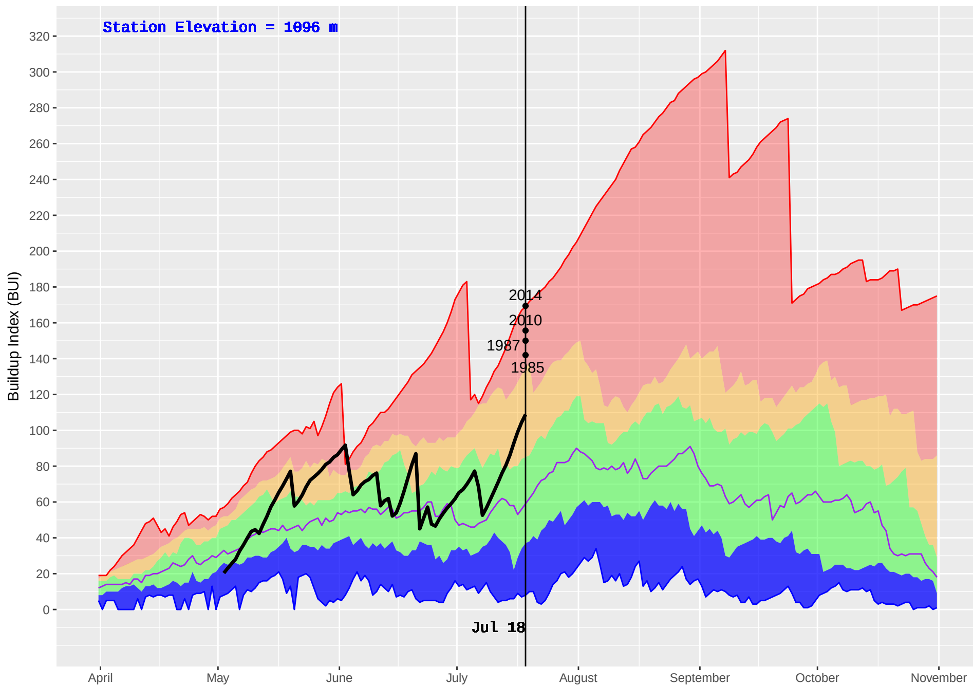
ANAHIM LAKE HUB (213) : Historical (1981–2016) and Current (2018) Daily Buildup Index (BUI)
